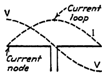
Current loop and current nodes on a half-wave doublet in free space.
